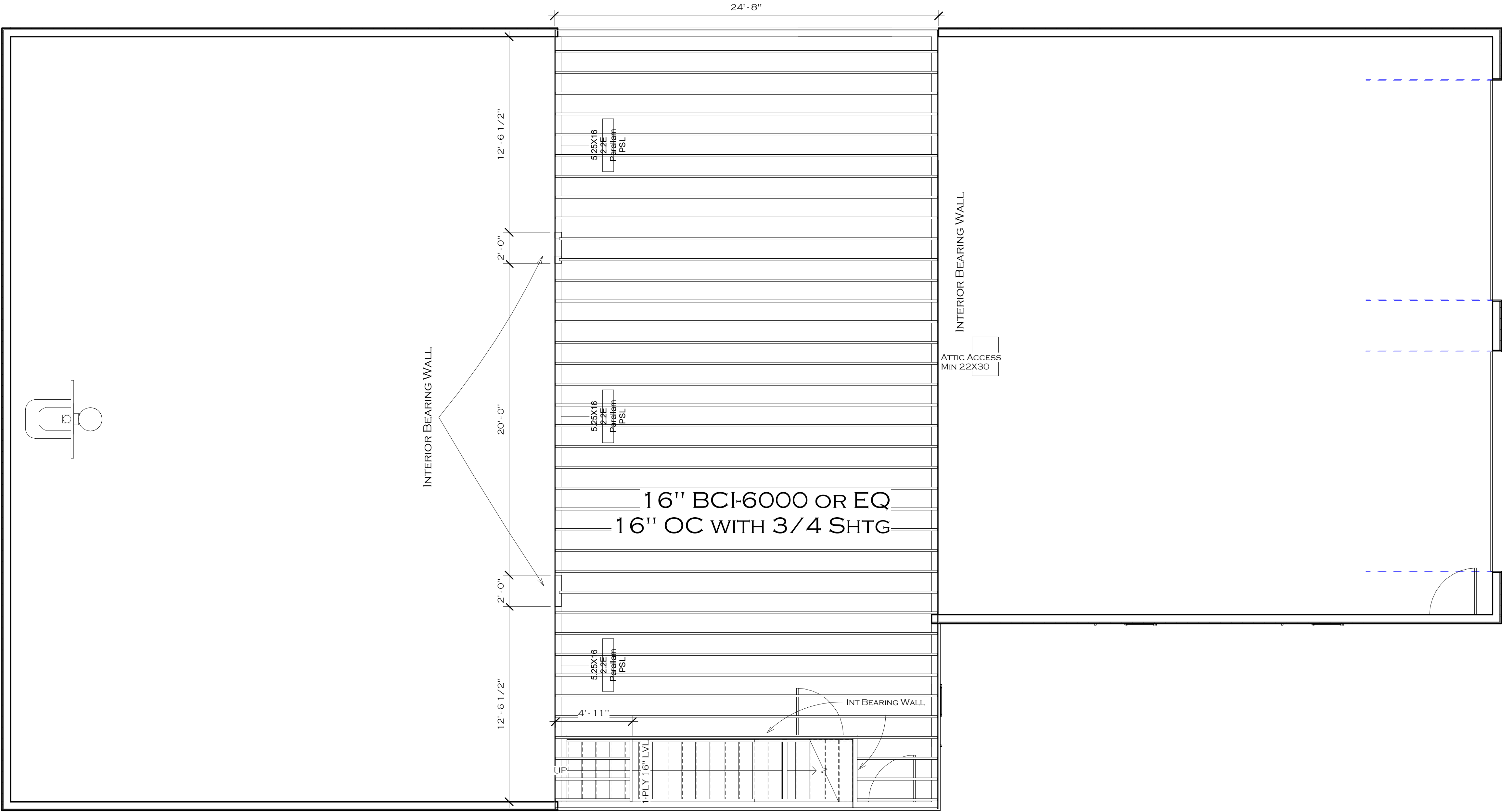
1 Balcony Framing 1/4" = 1'-0"
