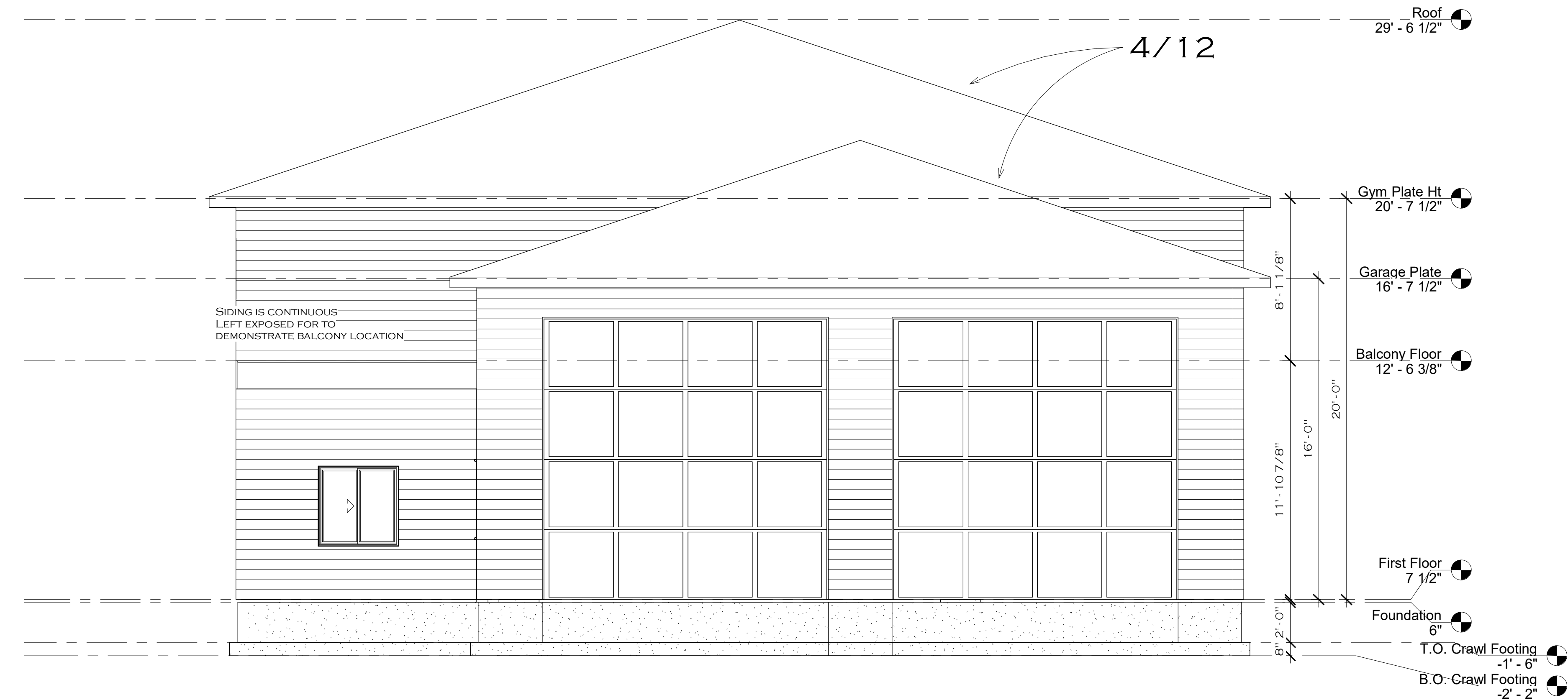
① Front 1/4" = 1'-0"
