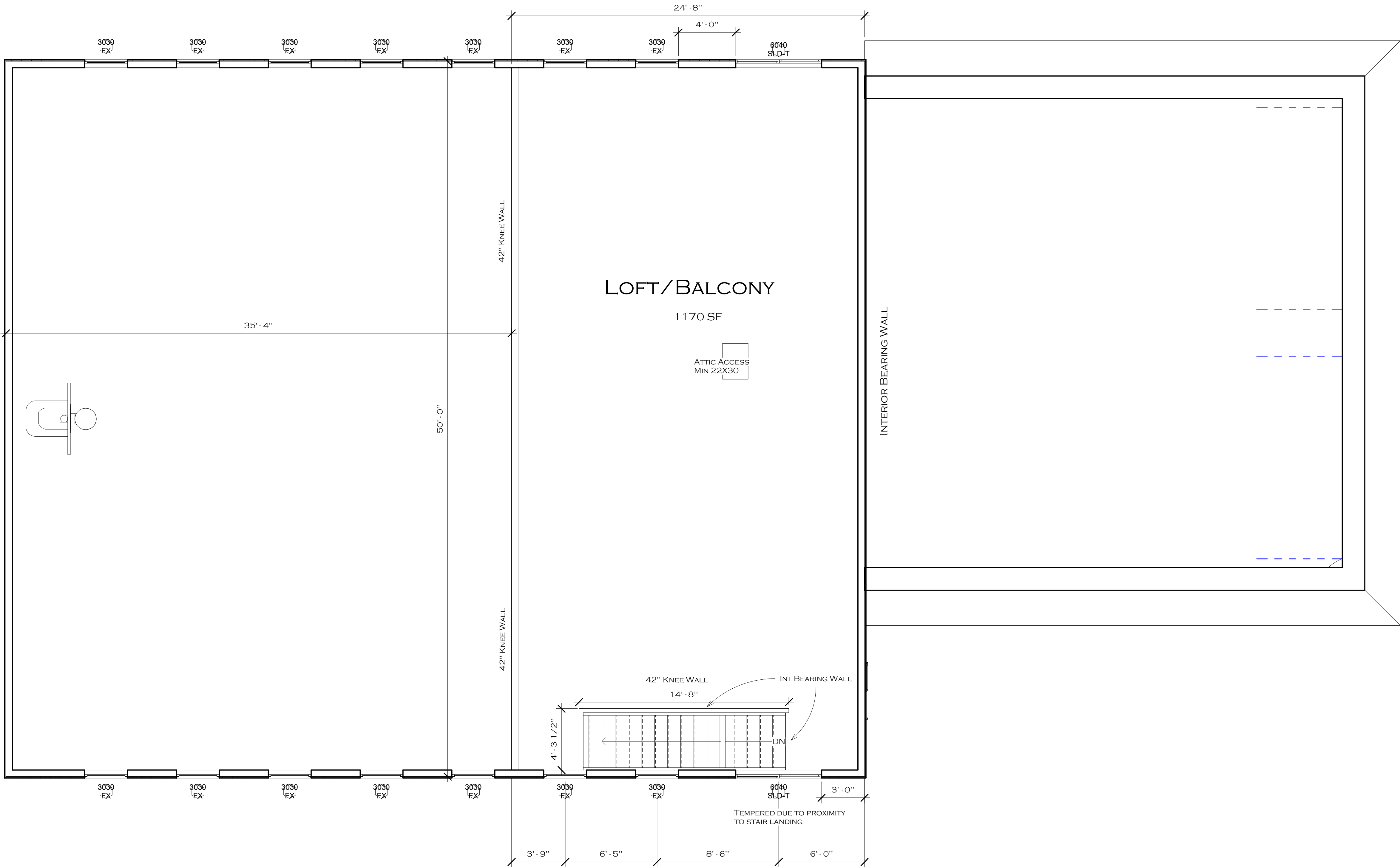
① Balcony Floor 1/4" = 1'-0"
